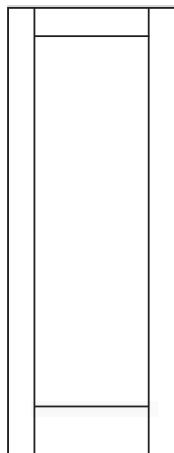
PR-C11 1 PANEL MDF, 6'8, 7'0 1-3/8" or 1-3/4" Square Sticking
